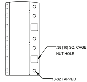
SCALE 1/2 FORWARD COMPATIBLE RACKRAIL
