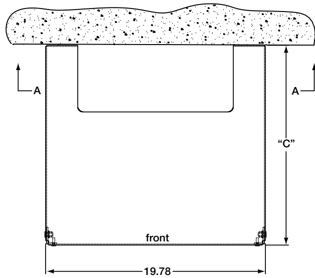
TOP/BOTTOM VIEW
